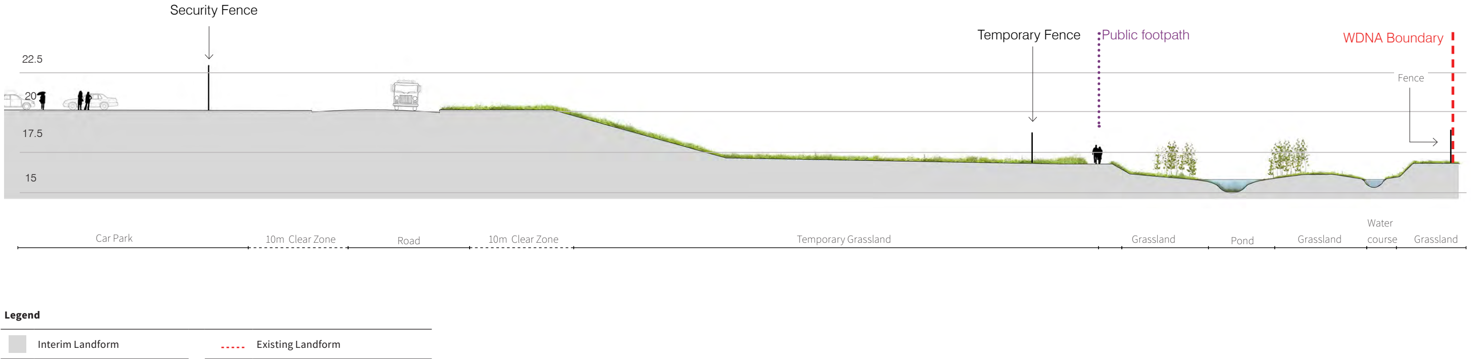
Figure 5-12 b - Illustrative sections of early planting during Main Construction
