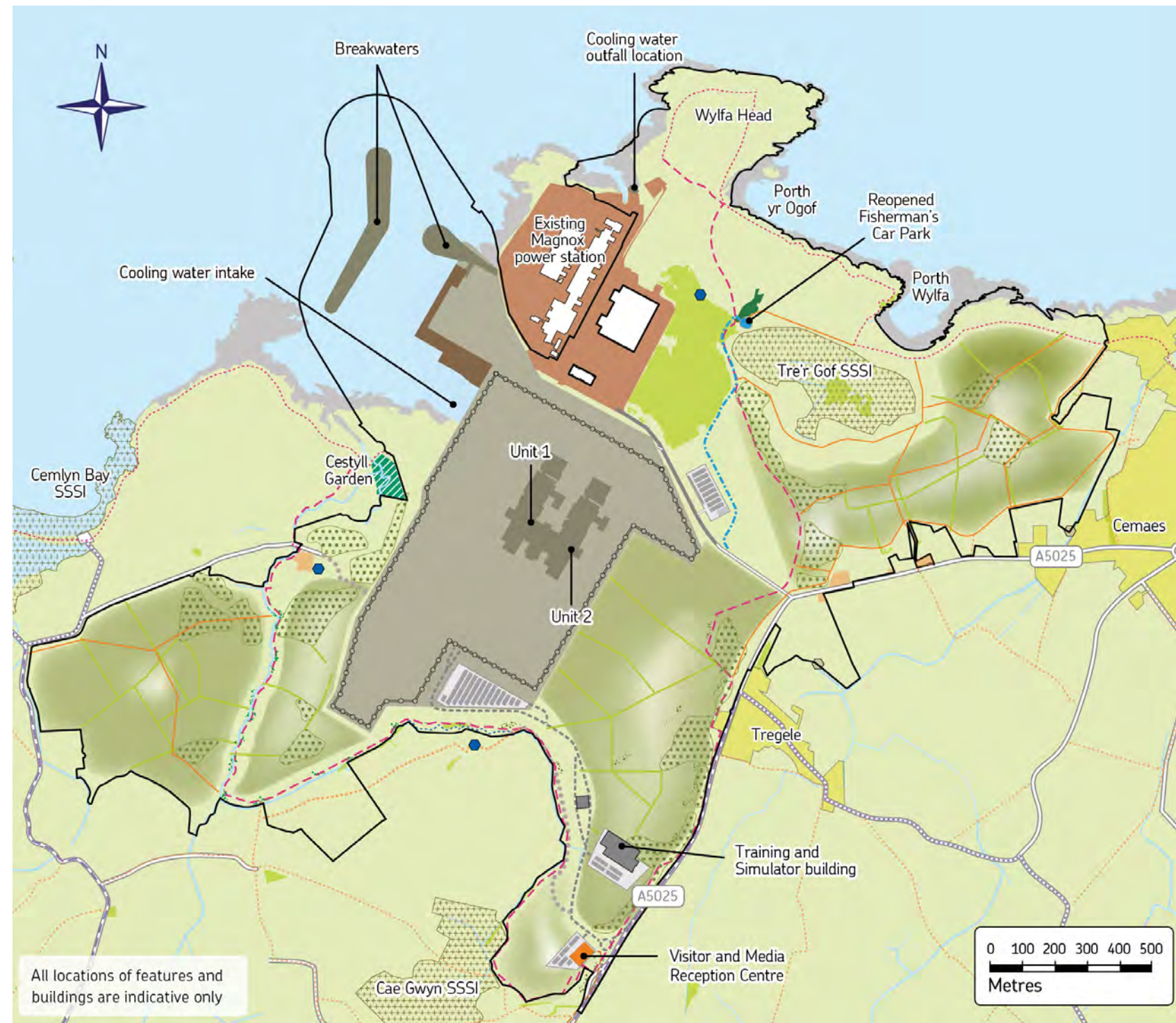
Figure 3-7 Landscape Setting – Stage Three Pre-Application Consultation
